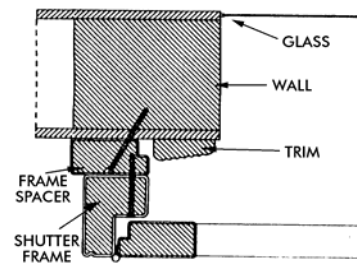
Install Beyond Trim
